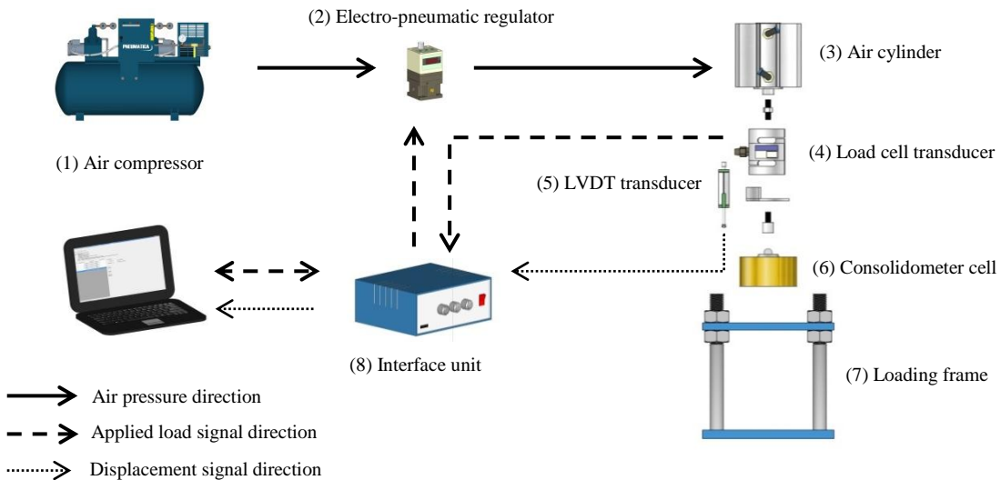
Fig.3 Structures of self-adjusted pneumatic loading one-dimensional Oedometer
