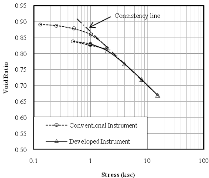
Fig. 9 Consolidation curve of traditional and automatic Oedometer
