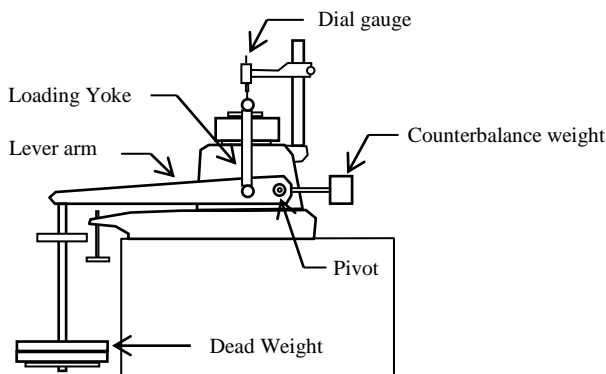
Fig. 1 one-dimensional Oedometer developed by Terzaghi
